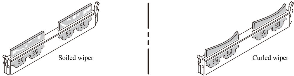
Examples of defective wiper
