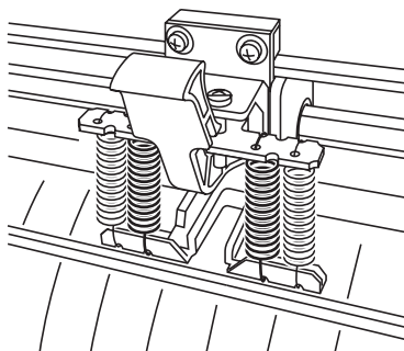
High mode : Raise the clamp pressure lever.
